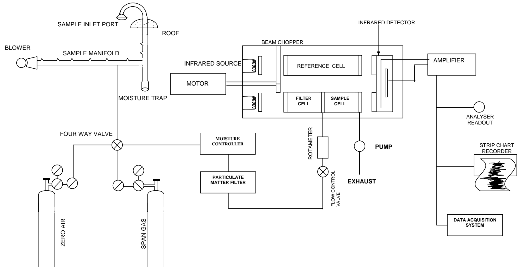
FIG : 1 TYPICAL CARBON MONOXIDE ANALYSER SYSTEM.
