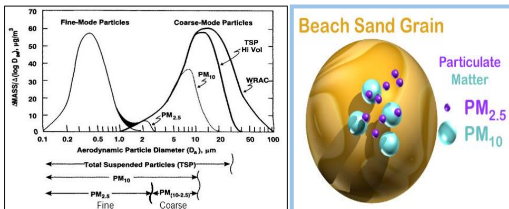
Figure 6.1: Particulate matter
