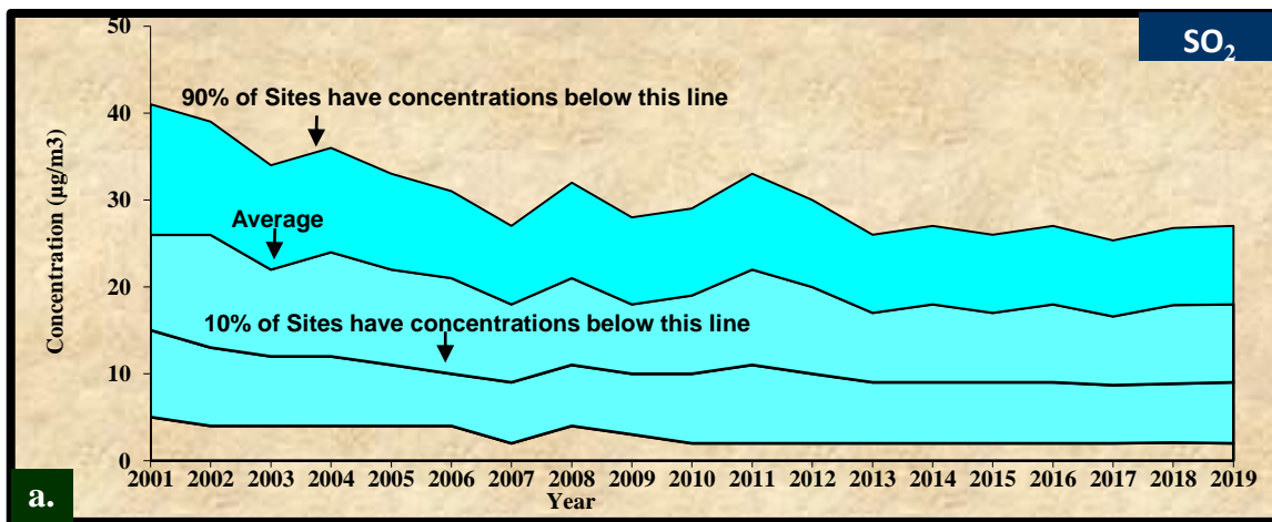
Figure 2.5: National mean concentration of different locations that fall under 10 th and 90 th Percentile for SO 2 , NO 2 , PM 10 and PM 2.5
