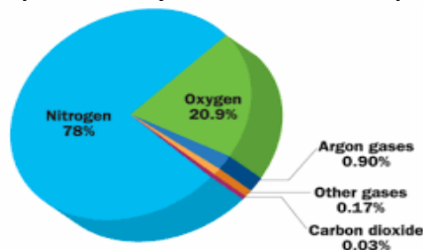
Figure 1.1: Composition of dry air in the lower atmosphere of the Earth
