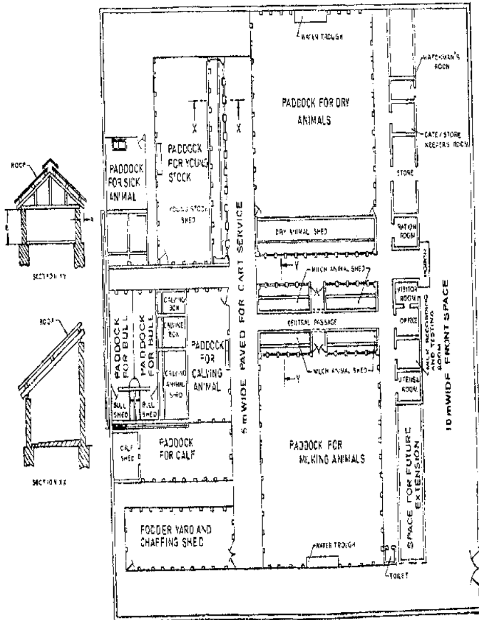
FIG. 1. TYPICAL LAYOUT OF FARM CATTLE SHED FOR GAUMHALAS' AND OTHER ORGANISED MILK PRODUCERS (Continued)
