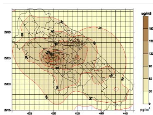
Isopleths for 24-hourly average- BAU-2007
