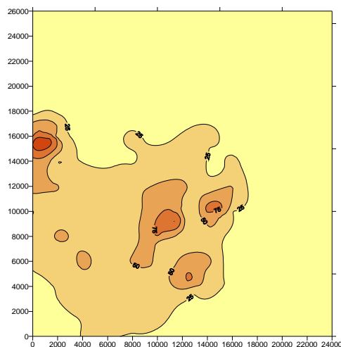
PM 10 Emission Load (Kg/day) – BAU-2007
