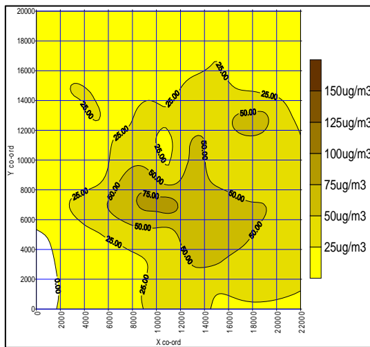
Isopleths for 24-hourly average– BAU-2007 PM 10 concentration (µg/m³)
