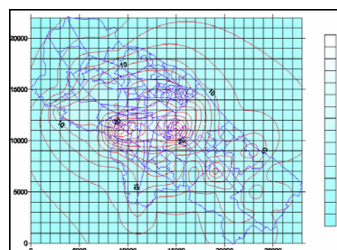
Isopleths for 24-hourly average- BAU-2007
