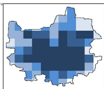
NO x Emission Load (Kg/day) – BAU-2007
