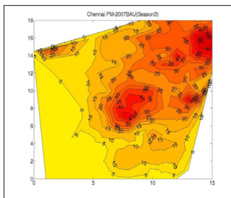
Isopleths for 24-hourly average- BAU-2007
