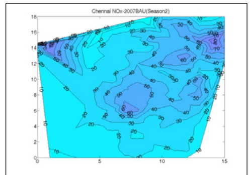
Isopleths for 24-hourly average– BAU-2007
