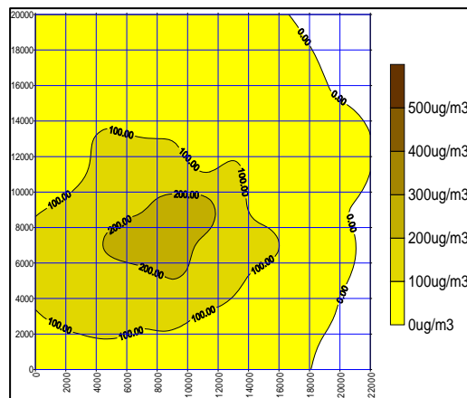
Isopleths for 24-hourly avg. PM 10 and NO x concentration ( \mu\text{g}/\text{m}^3 ) respectively for winter:
