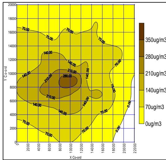
Isopleths for 24-hourly avg. PM 10 and NO x concentration ( \mu\text{g}/\text{m}^3 ) respectively for winter: 2012BAU
