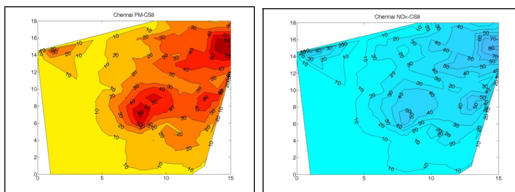
Isopleths for 24-hourly avg. PM_{10} and NO_x concentration ( \mu g/m^3 ) respectively for Post Monsoon: Control Scenario 2012
