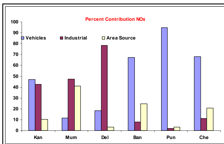
Figure 4.5: Prominence of Sources of NO x
