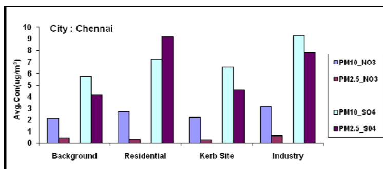
Figure 3.20: EC/OC and \text{SO}_4^{2-}/\text{NO}_3^- , in \text{PM}_{10}/\text{PM}_{2.5} in Chennai
