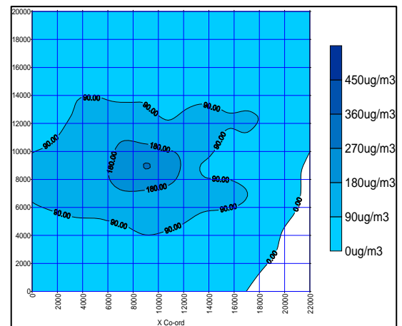
Isopleths for 24-hourly avg. PM 10 and NO x concentration ( \mu\text{g}/\text{m}^3 ) respectively for winter:
