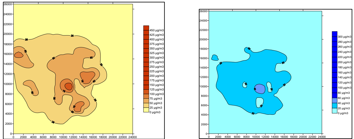
Isopleths for 24-hourly avg. PM 10 and NO x concentration (µg/m 3 ) respectively for winter: Control Scenario 2017
