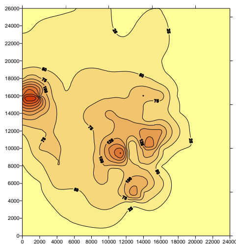
PM 10 concentration (µg/m 3 )
