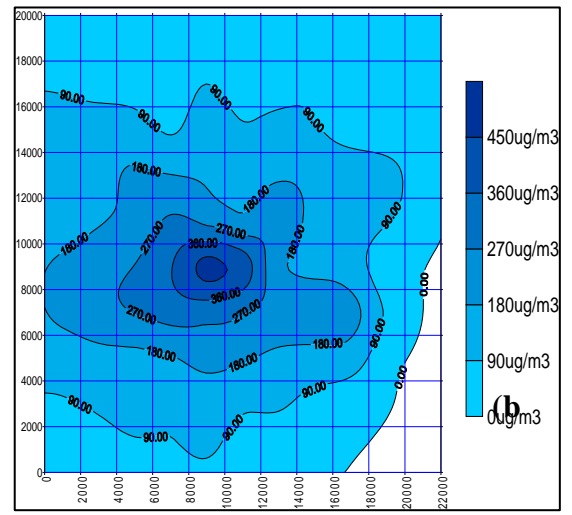
Isopleths for 24-hourly avg. PM 10 and NO x concentration ( \mu\text{g}/\text{m}^3 ) respectively for winter: 2012BAU
