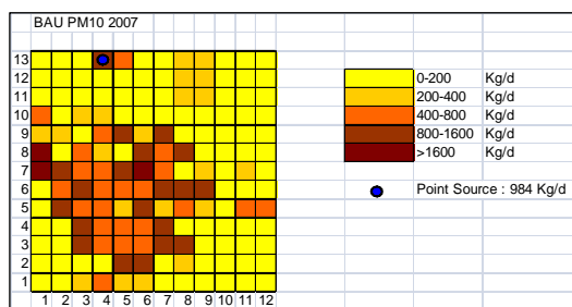
PM 10 Emission Load (Kg/day) – BAU-2007
