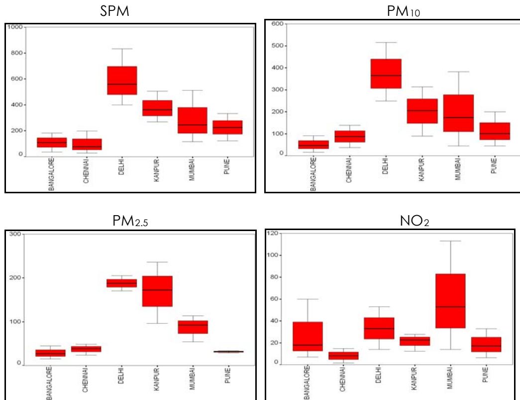
Figure 3.5: Box plots of SPM, PM 10 , PM 2.5 and NO 2 Concentrations (in \mu\text{g}/\text{m}^3 ) at Background Locations
