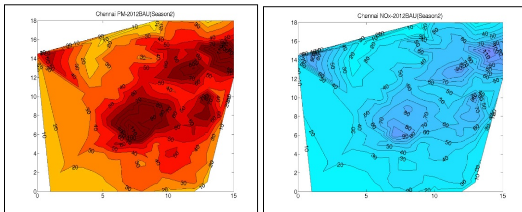
Isopleths for 24-hourly avg. PM_{10} and NO_x concentration ( \mu g/m^3 ) respectively for Post Monsoon: 2012 BAU
