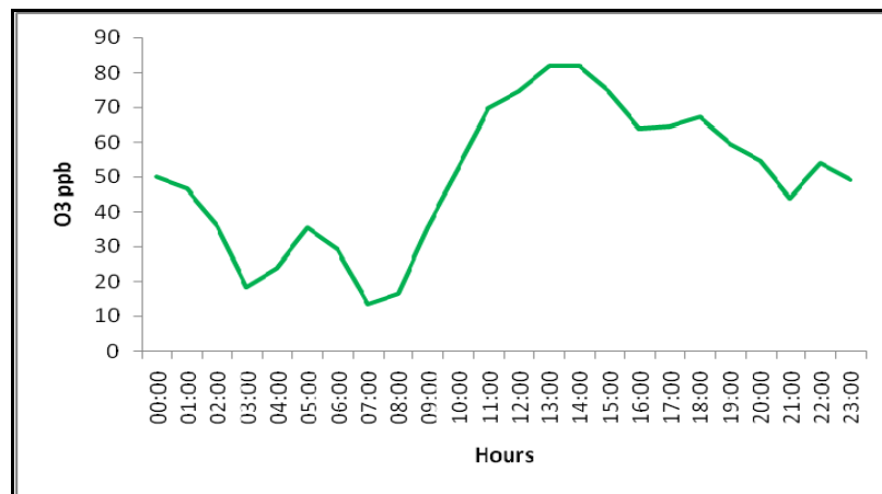
Figure 3.17: Temporal variation of O 3 concentration in Mumbai
