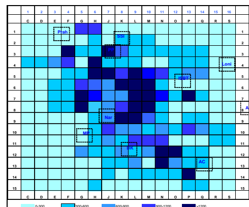
NO x Emission Load (Kg/day) – BAU-2007
