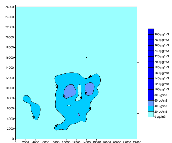
Isopleths for 24-hourly average– BAU-2007
