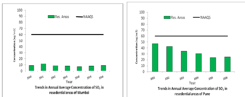
Figure 3.3: Air Quality Trends of SO 2 in Residential Areas
